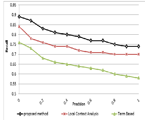
Fig3. Recall/Precision of The proposed Approach in IR
