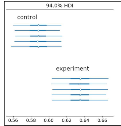
Fig. 6. 94% HDI sample comparison for sklearn score.
