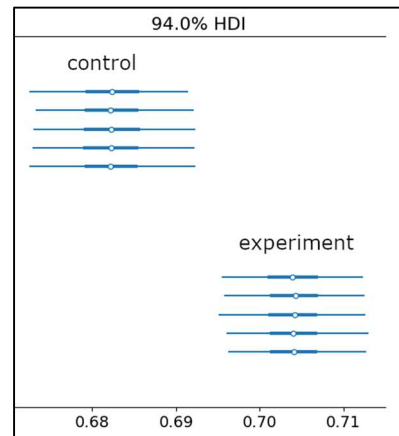
Fig. 7. 94% HDI sample comparison for BERTscore.
