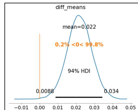
Fig. 9. Posterior distribution of the difference of means for the BERTscore.
